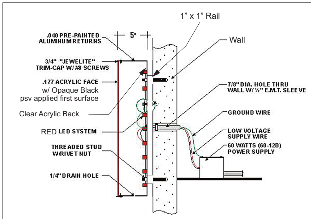
Typical Rail Mounted Reverse Channel Letter
