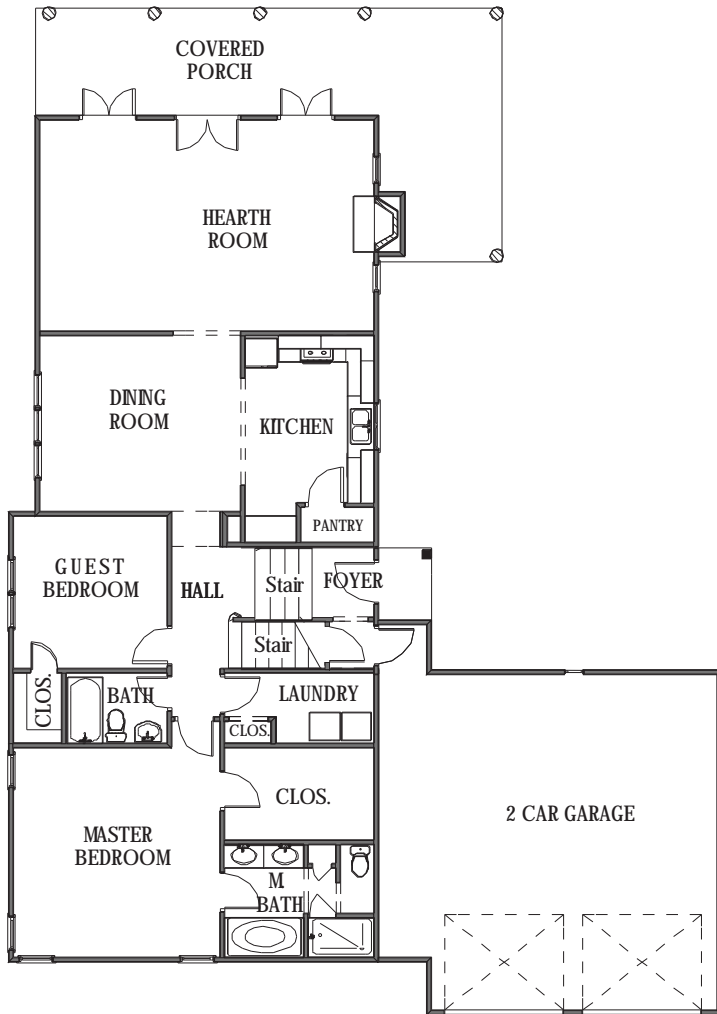
First Floor not to scale
