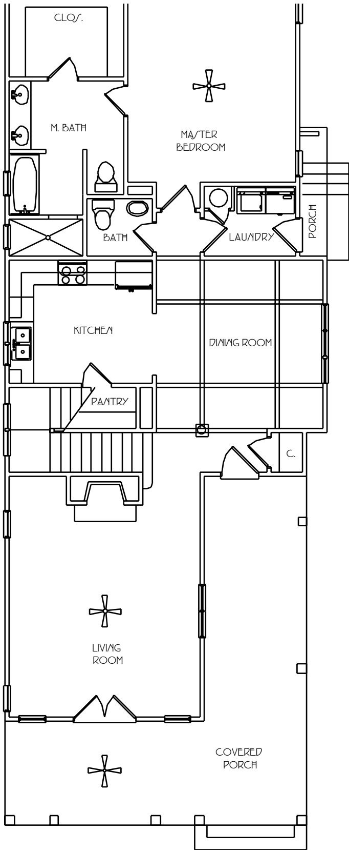
First Floor not to scale
