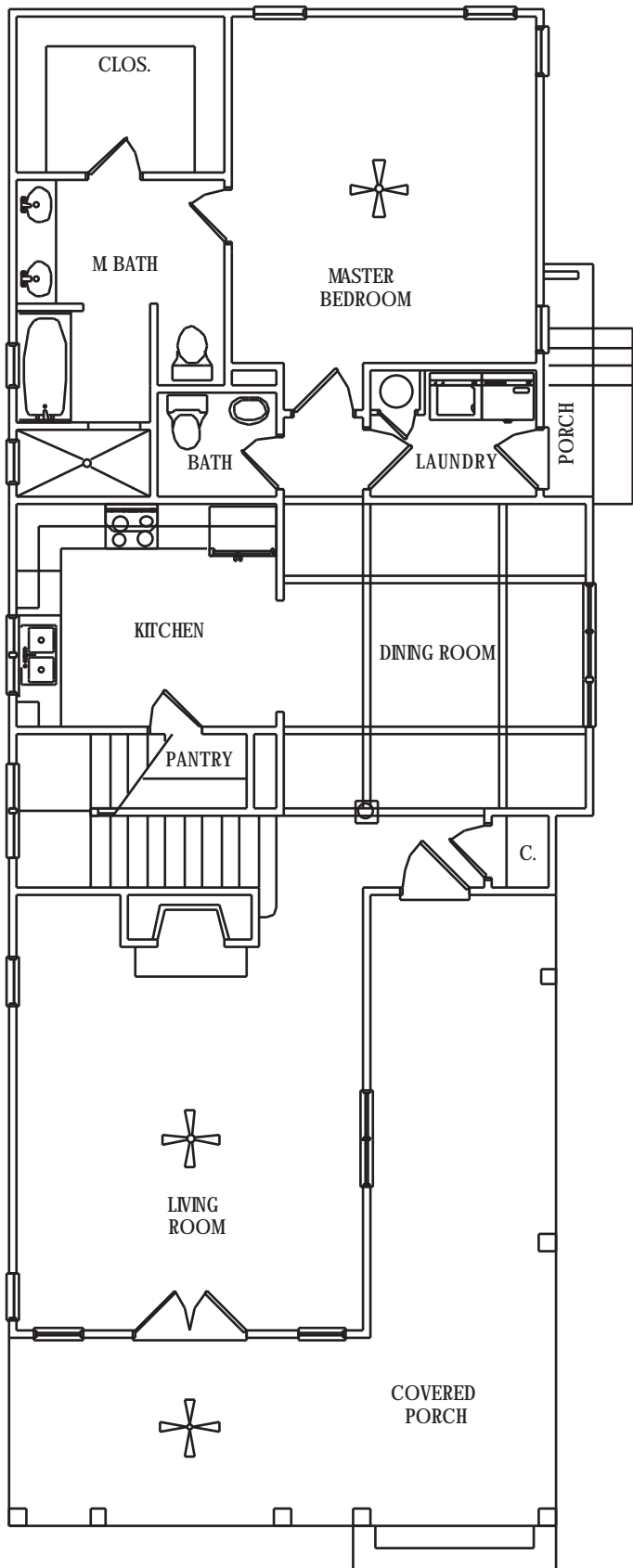
First Floor not to scale
