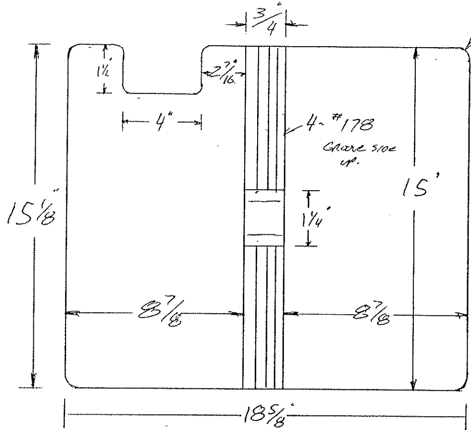
TOP VIEW OF DIE
