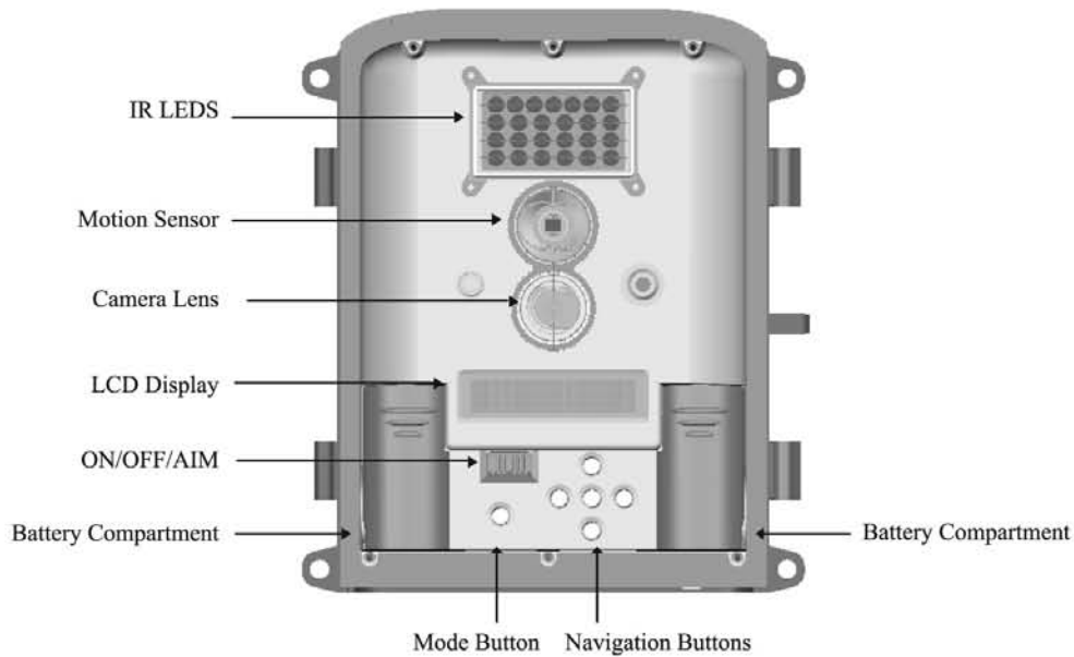
BOTTOM VIEW
